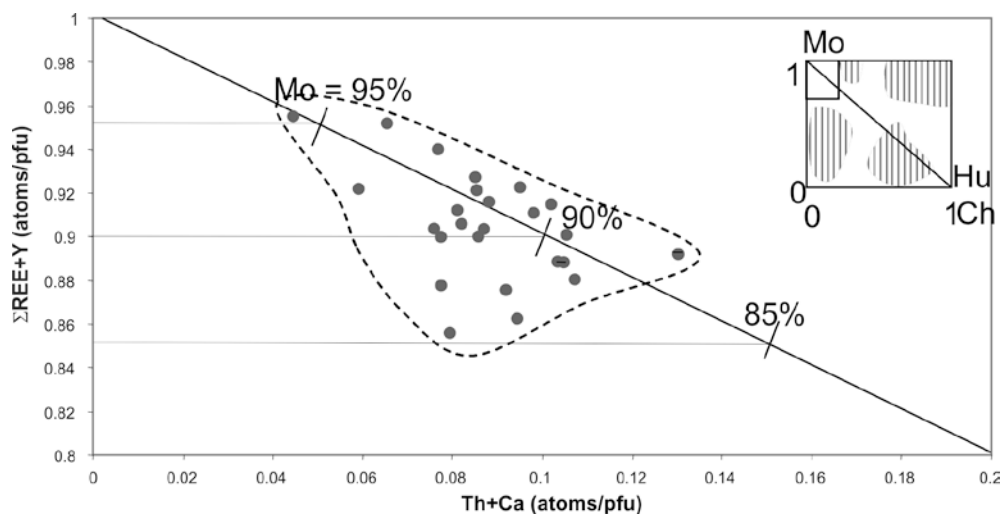
Figure 5. Composition of monazite-(Ce) in \Sigma\text{REE}+\text{Y}/\text{pfu} - \text{Th}+\text{Ca}/\text{pfu} diagram after Broska et al., 2000
